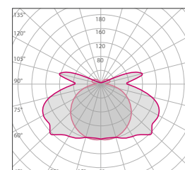
Curva fotometrica Photometric diagram
